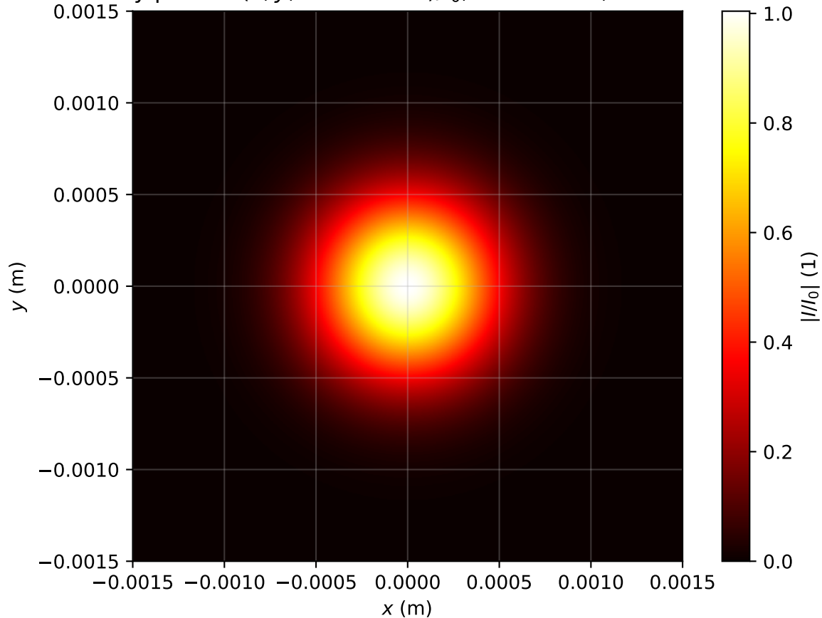
Intensity profile I(x, y, z = 0.080\text{m})/I_0 , \text{Pin}=0.9\text{Pcr} , artificial time
